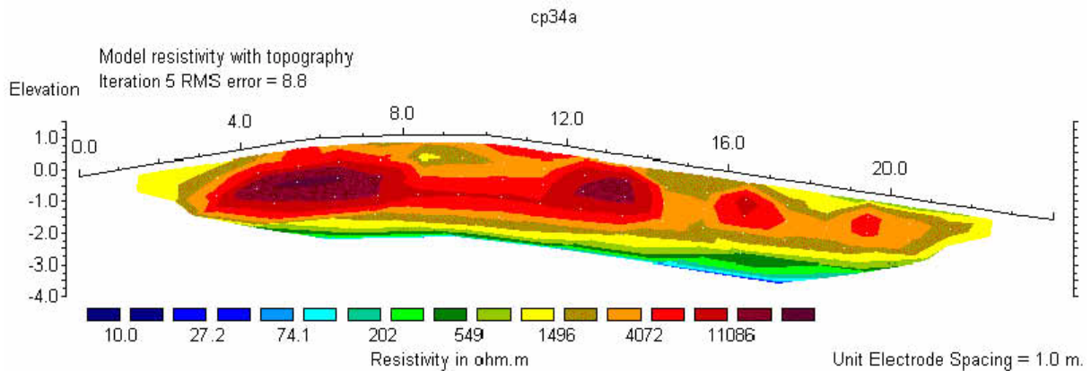
Illus 8 Capo Barrow: (a) Profile 34, measured apparent resistivities and topography used in modelling the profiles (scale altered to accommodate larger variations seen in the model [8c]); (b) Profile 34, apparent resistivities calculated from the model; (c) Profile 34, modelled resistivity cross-section with true depth scale. North at left side of plots
