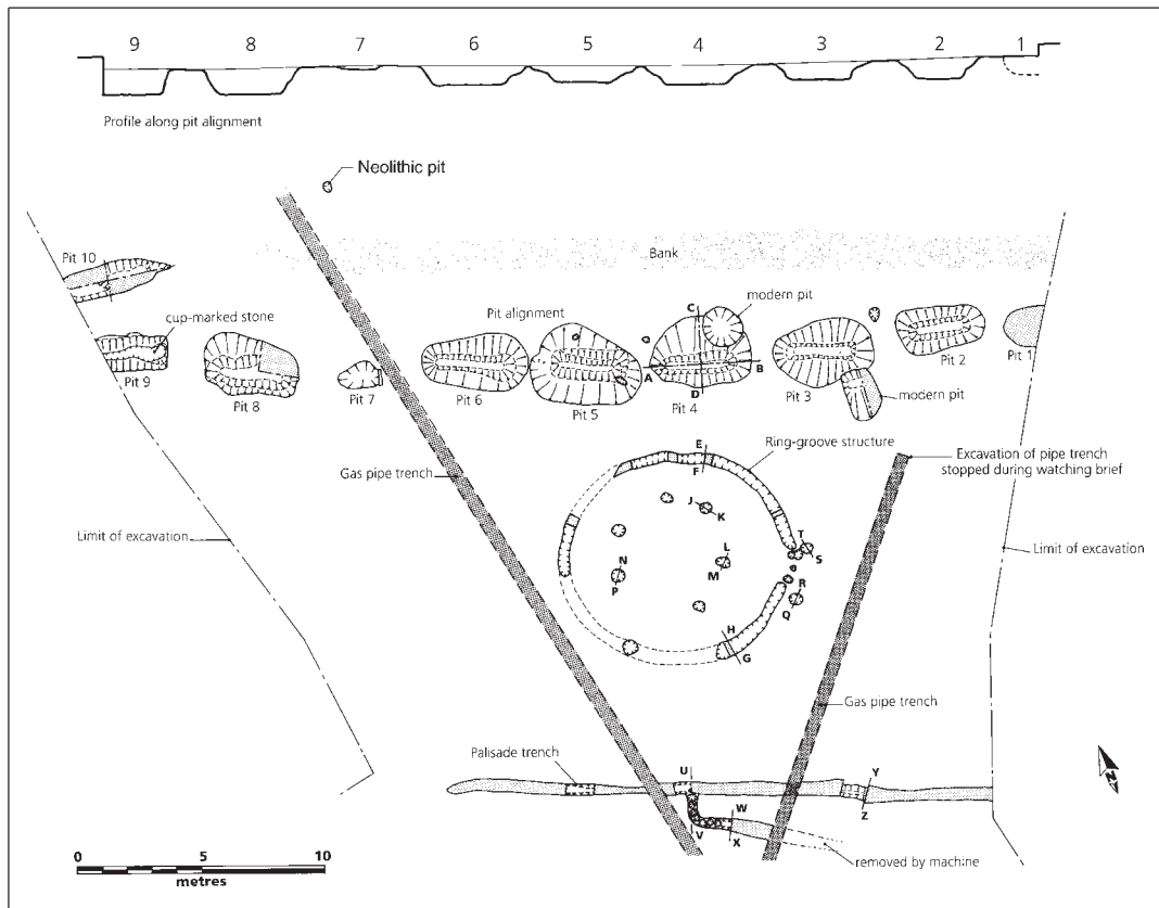
ILLUS 6 Neolithic pit, late prehistoric features and section locations
