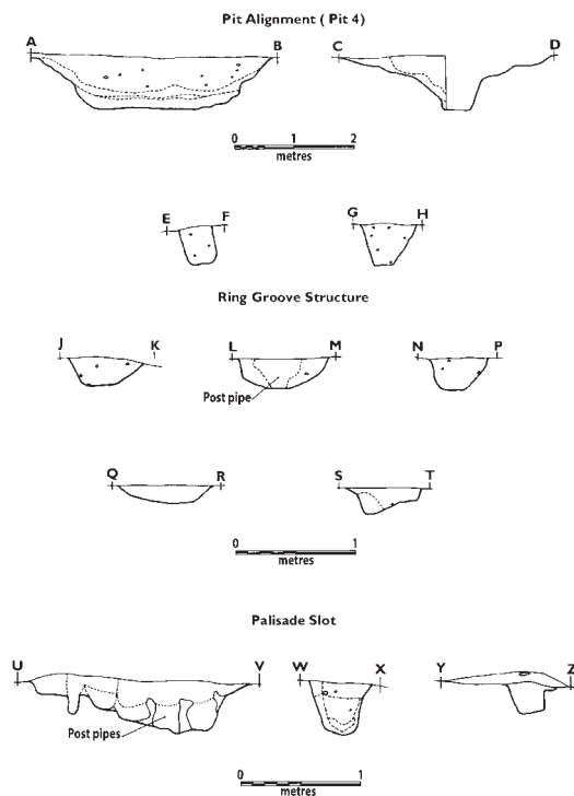
ILLUS 13 Pit 4, ring-groove and palisade sections
