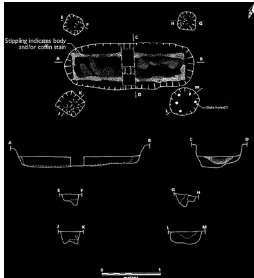
ILLUS 38 Plan, profiles and section of Grave 16
