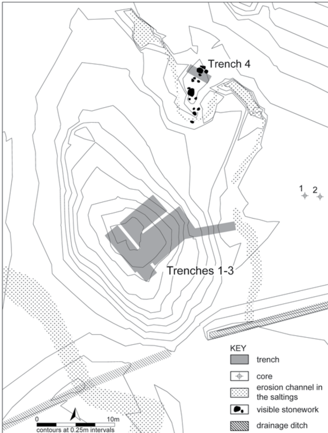
ILLUS 3 Pre-excavation survey and plan, showing location of trenches
