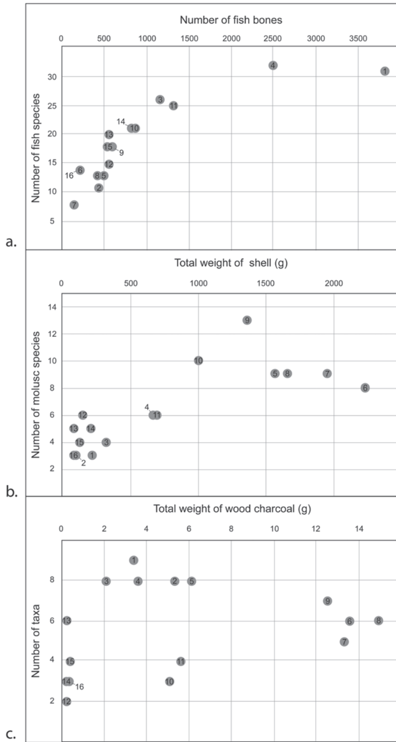
ILLUS 15 The relationship between species/taxa frequency and sample size for (a) fish bones, (b) mollusc shell, and (c) wood charcoal
