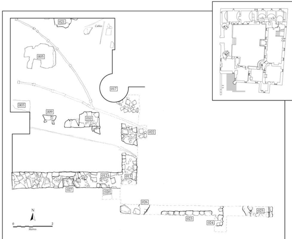
ILLUS 12 Plan of the excavation on the site of the south wing
