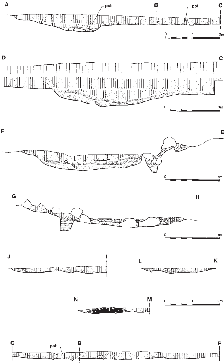
ILLUS 9 Deer's Den: Structure 3 sections
