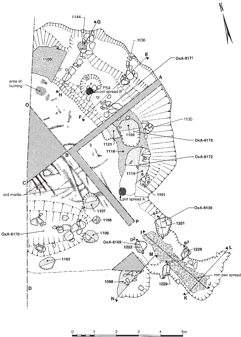
ILLUS 8 Deer's Den: plan of Structure 3
