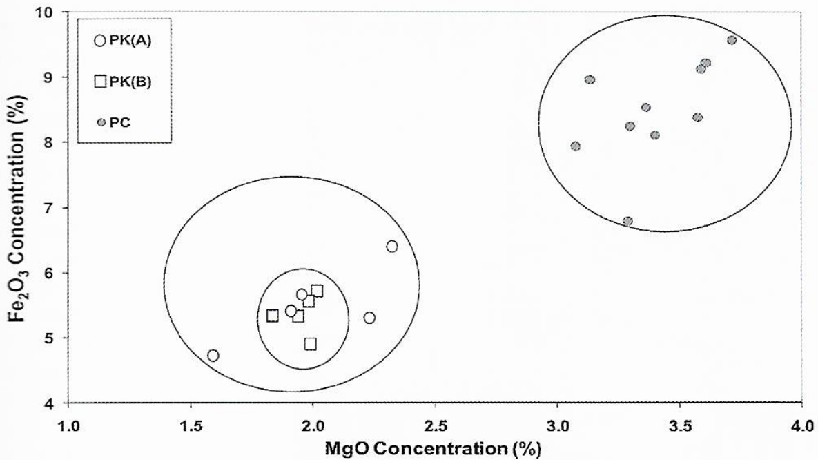
ILLUS 11 Bi-variate plot of MgO and Fe 2 O 3 concentrations demonstrating the differences between Perth Canal Street (PC) and either Perth Kinnoull (PK(A) and PK(B))
